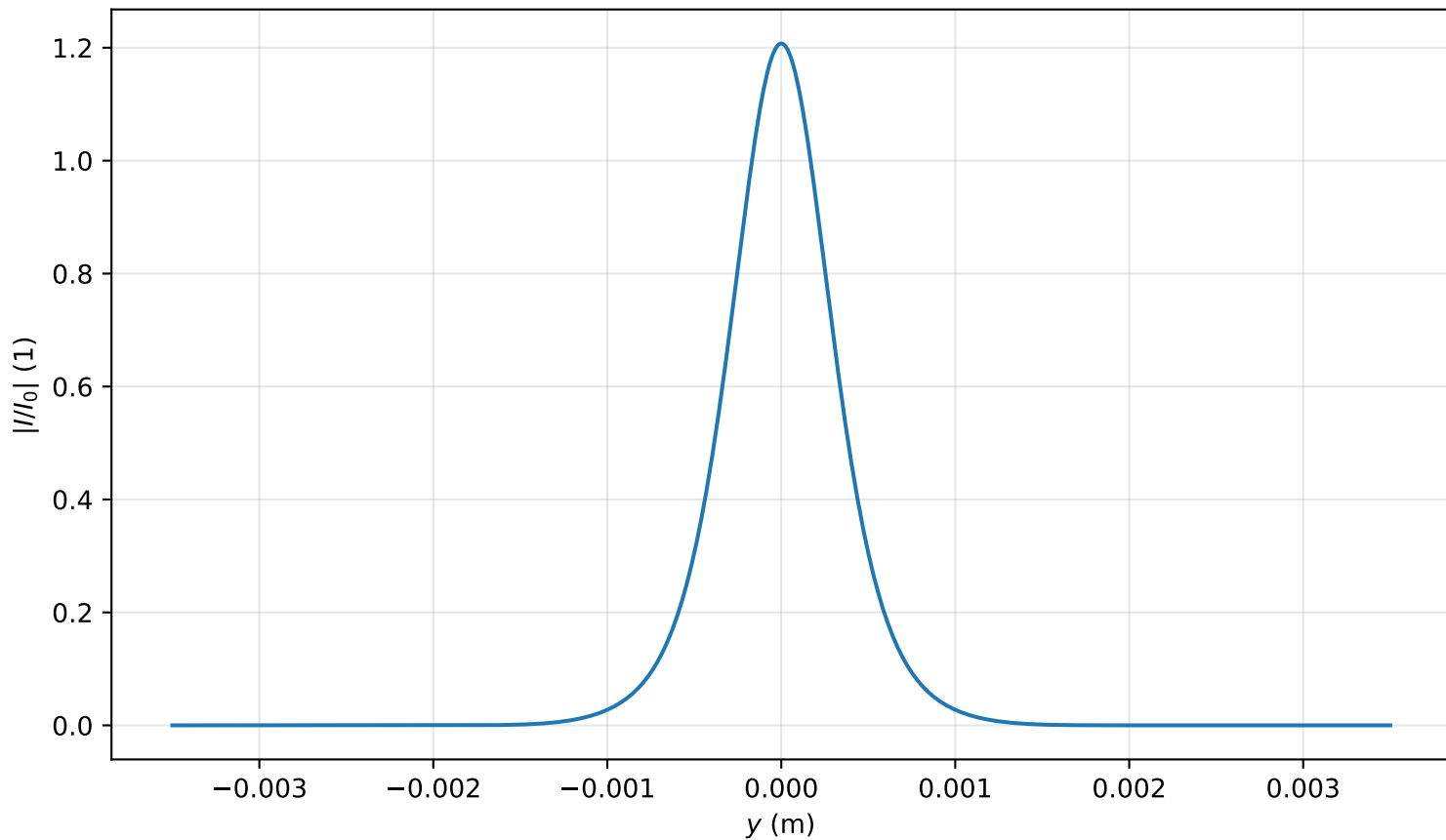
Intensity profile I(x=0, y, z=1.353)/I_0 , P_{in}=0.7P_{cr} , artificial time
